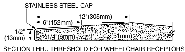
SECTION THRU THRESHOLD FOR WHEELCHAIR RECEPTORS
