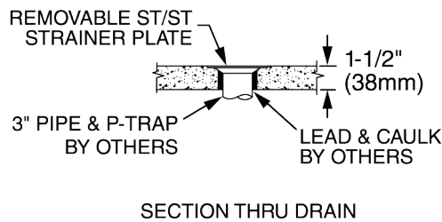
SECTION THRU DRAIN
