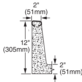
Series TSB200 With Plain Curbs
