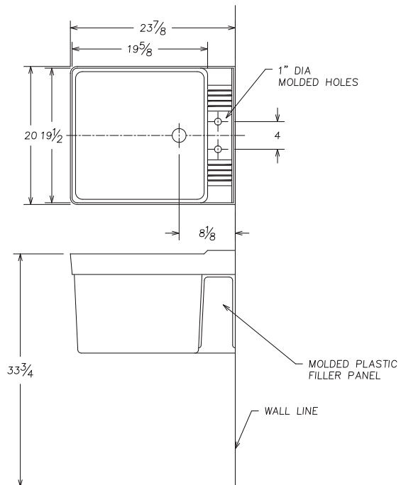
SF1W Wall Hung Tuf-Tub™
