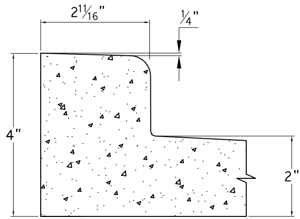
SECTION THRU THRESHOLD SECTION 2
