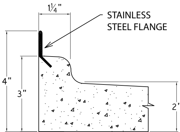
SECTION THRU SIDE SECTION 1
